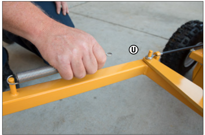
16. Attach spring to groove on jaw assembly pin U .
