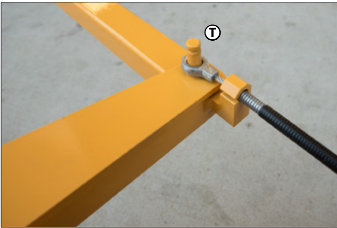
15. Install cable clip onto jaw assembly pin T .
